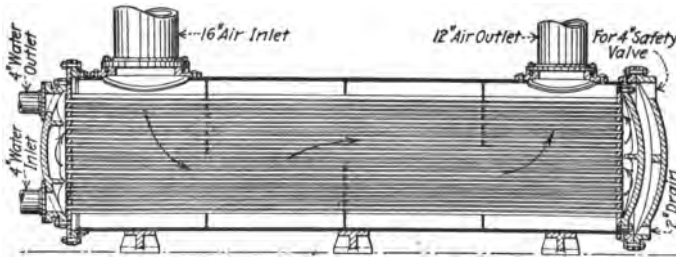
FIG. 127.—Receiver aftercooler.
